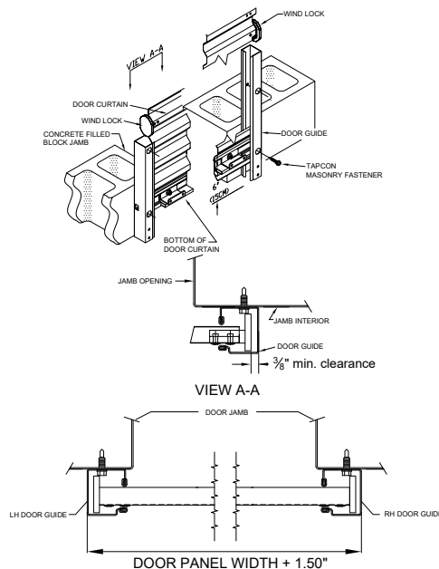
Figure 7 Windlock Door
