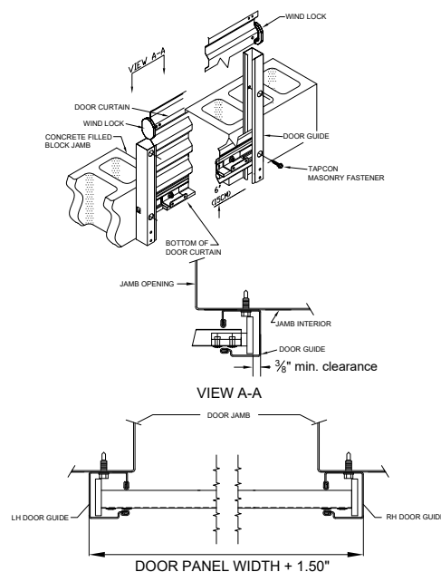
Figure 7 Windlock Door
