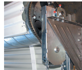
Chain hoist mounts directly to the axle for easy installation. 8:1 reduced-drive allows for smooth operation.
